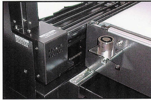
Linear bearings allow sealer to easily move forward or backward to center package into tunnel.
